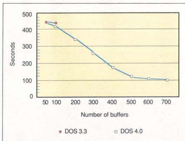
Figure 2: The performance improvements from using large buffers with 12,800 random-sector reads and writes on a 256K-byte file. The test was done on a PS/2 Model 60.
